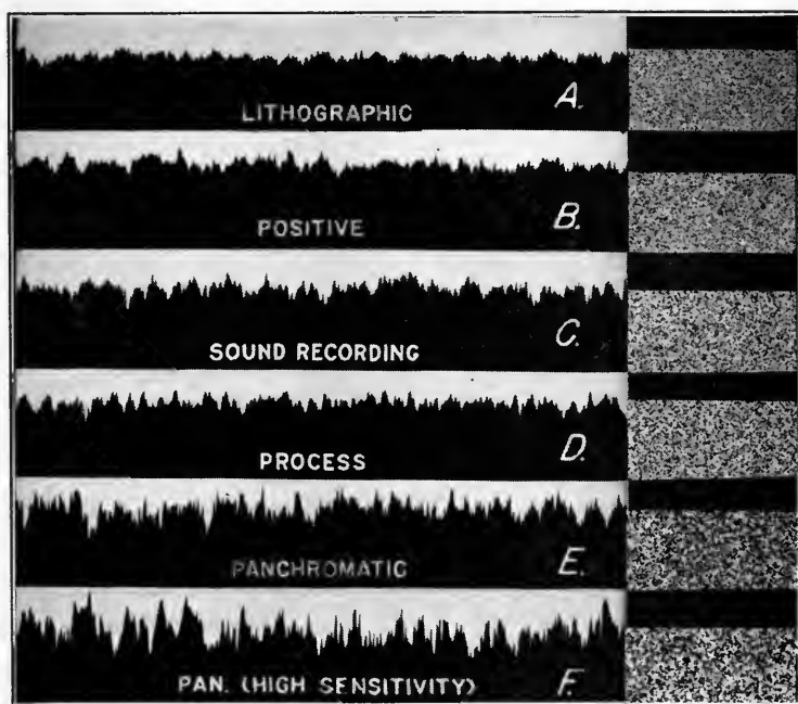
FIG. 5. Graininess records of six different emulsions of nearly equal density. On the right, photomicrographs of emulsions (300 diam.) for comparison of objective and subjective graininess.
